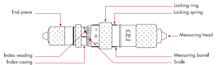
MICROMETER HEAD - M130
